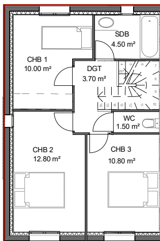
VILLA 1 / R+1 Ech: 1/150
